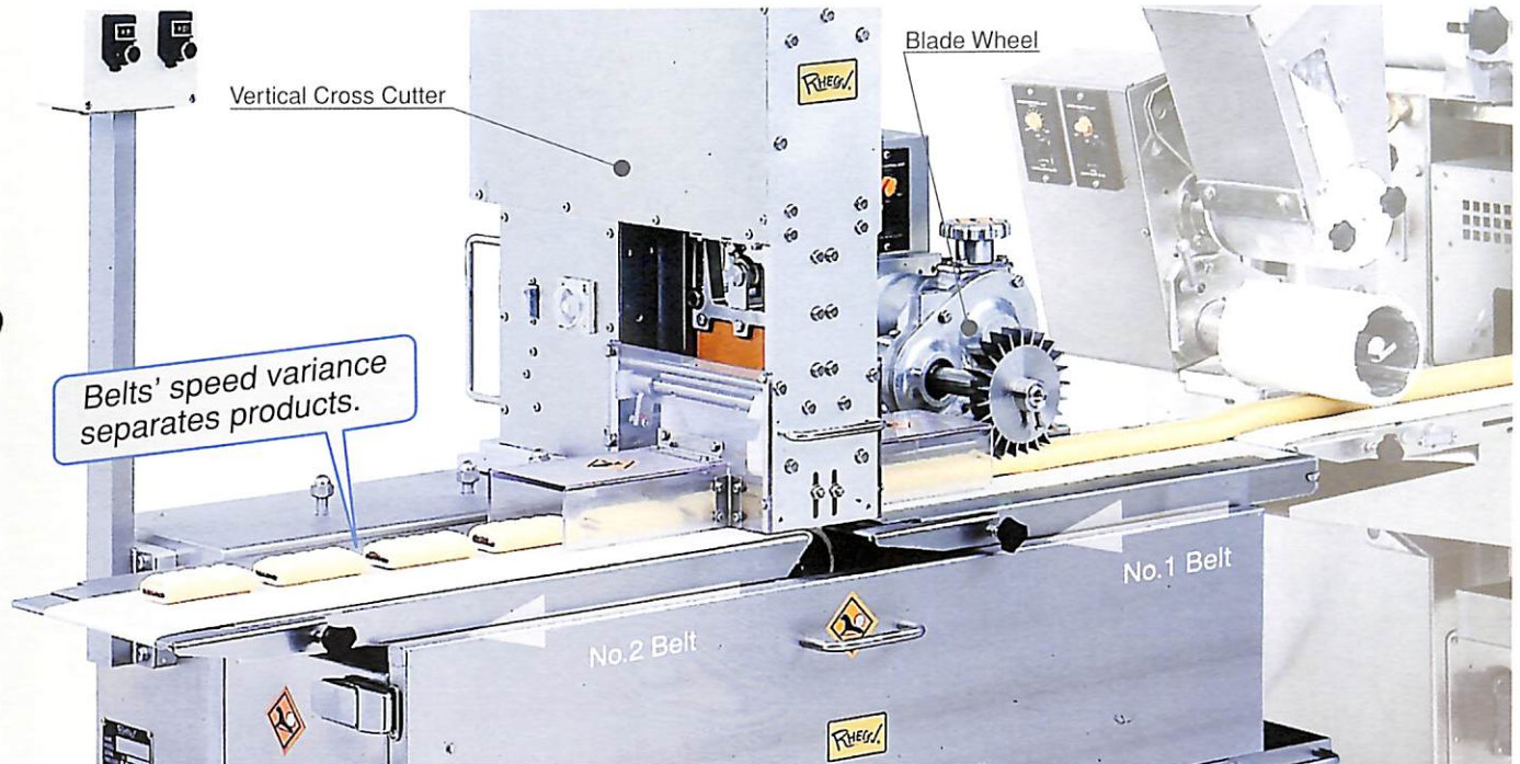
▲ Example of shaping options (Blade Wheel and Vertical Cross Cutter are covered with safety covers on operation)
